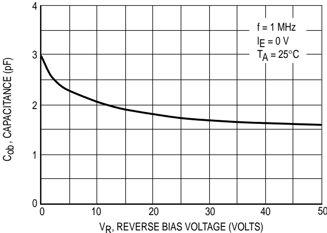
Figure 9. Output Capacitance
