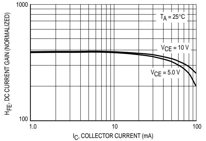
Figure 43. DC Current Gain — NPN
