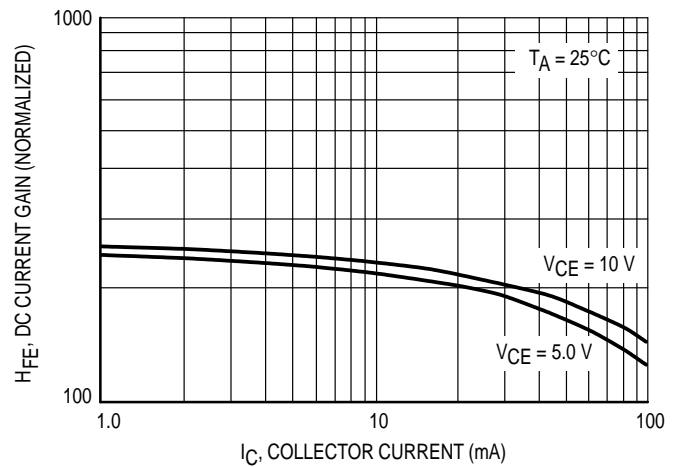
Figure 45. DC Current Gain — NPN
