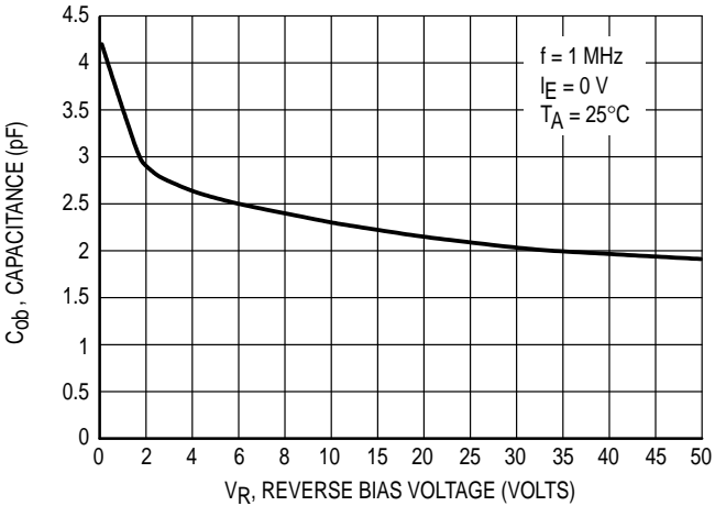
Figure 39. Output Capacitance
