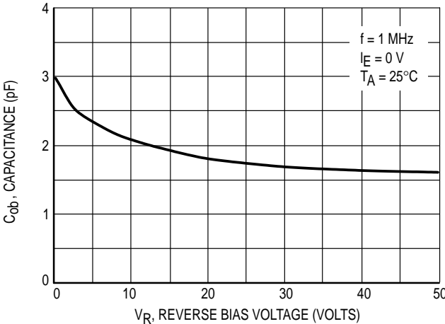
Figure 19. Output Capacitance
