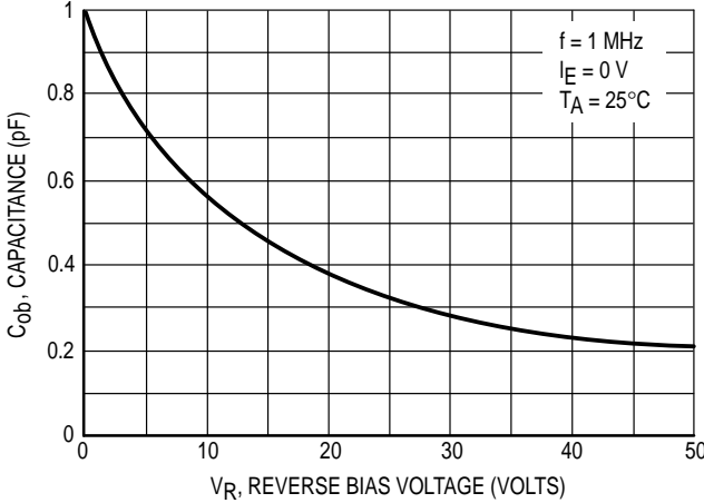
Figure 29. Output Capacitance
